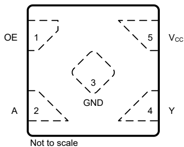
Figure 4-1. DTX Package, 5-Pin X2SON (Top View)
