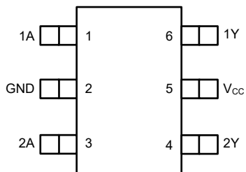
Figure 4-1. DBV, 6-Pin SOT-23 (Top View)
