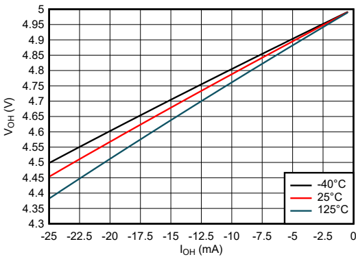
Figure 5-4. Output Voltage vs Current in HIGH State; 5V Supply
