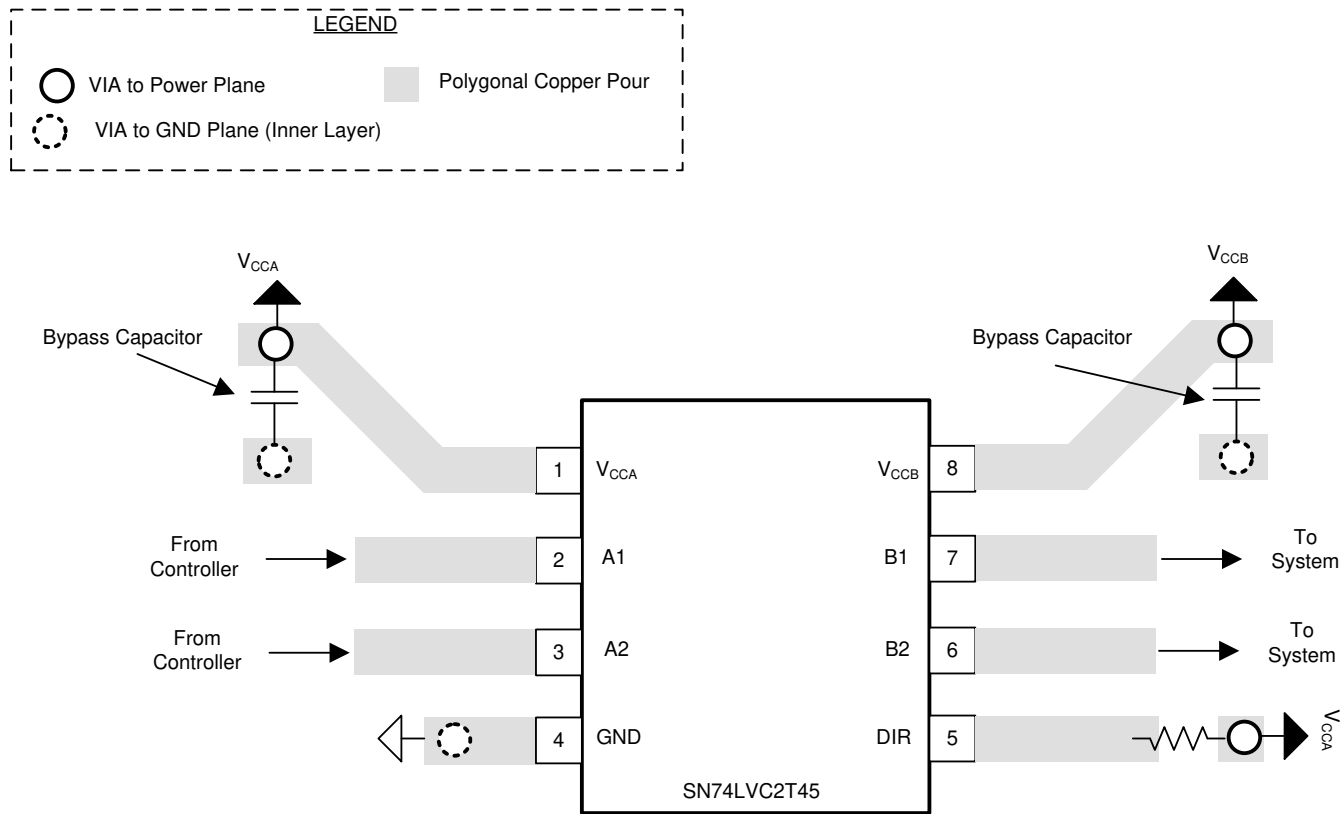
Figure 8-3. SN74LVC2T45 Layout Example
