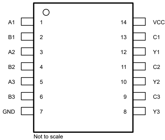
Figure 4-1. SN74LVC3G98-Q1 PW Package (Preview), 14-Pin TSSOP (Top View)
