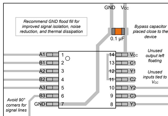
Figure 8-3. Example Layout for the SN74LVC3G98-Q1
