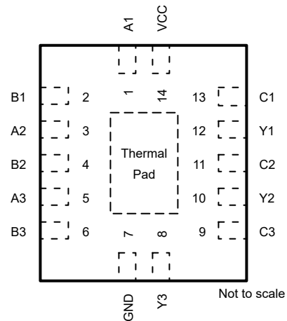
Figure 4-2. SN74LVC3G98-Q1 BQA Package, 14-Pin WQFN (Top View)
