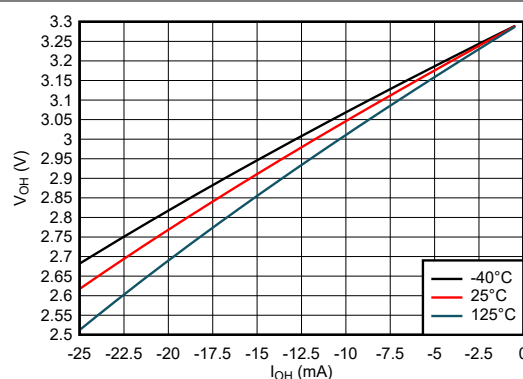
Figure 5-2. Output Voltage vs Current in HIGH State; 3.3V Supply
