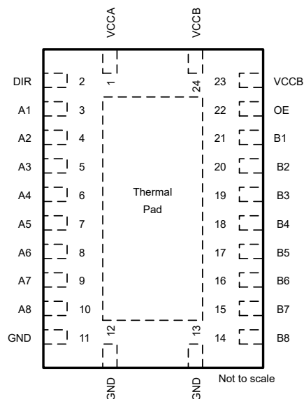
Figure 4-2. RHL Package, 24-Pin VQFN (Top View)
