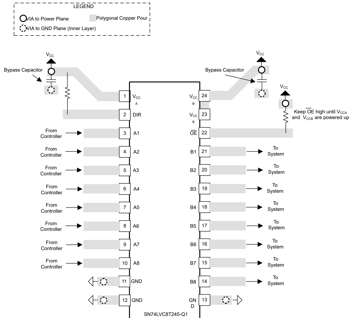
Figure 8-3. SN74LVC8T245 Layout
