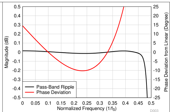
Figure 6-56. Ultra-Low-Latency Decimation Filter Pass-Band Ripple and Phase Deviation
