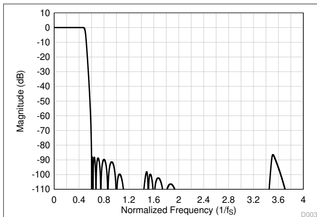
Figure 6-55. Ultra-Low-Latency Decimation Filter Magnitude Response
