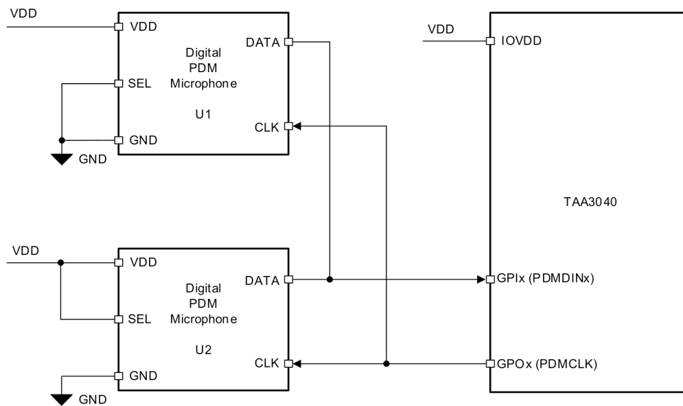
Figure 6-64. Digital PDM Microphones Connection Diagram to the TAA3040
