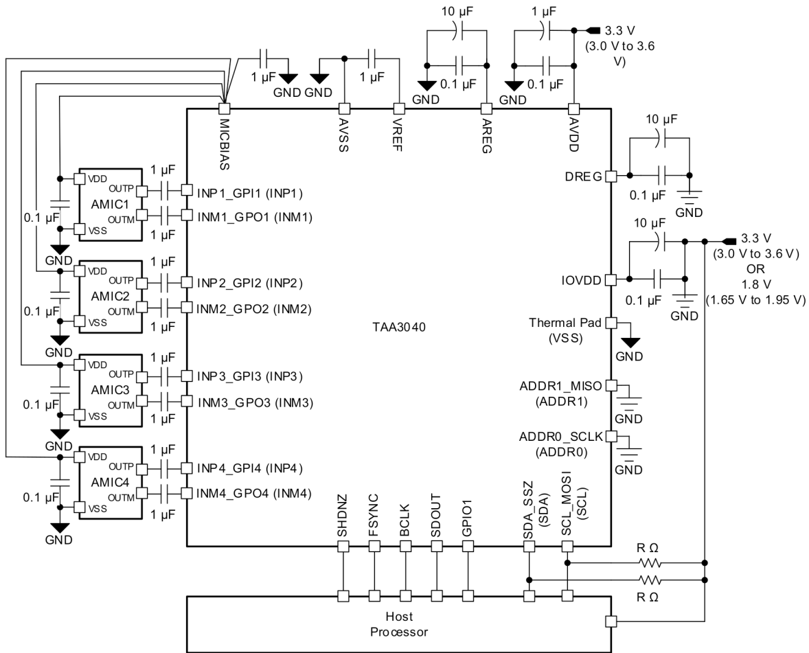
Figure 8-1. Four-Channel Analog Microphone Recording Diagram
