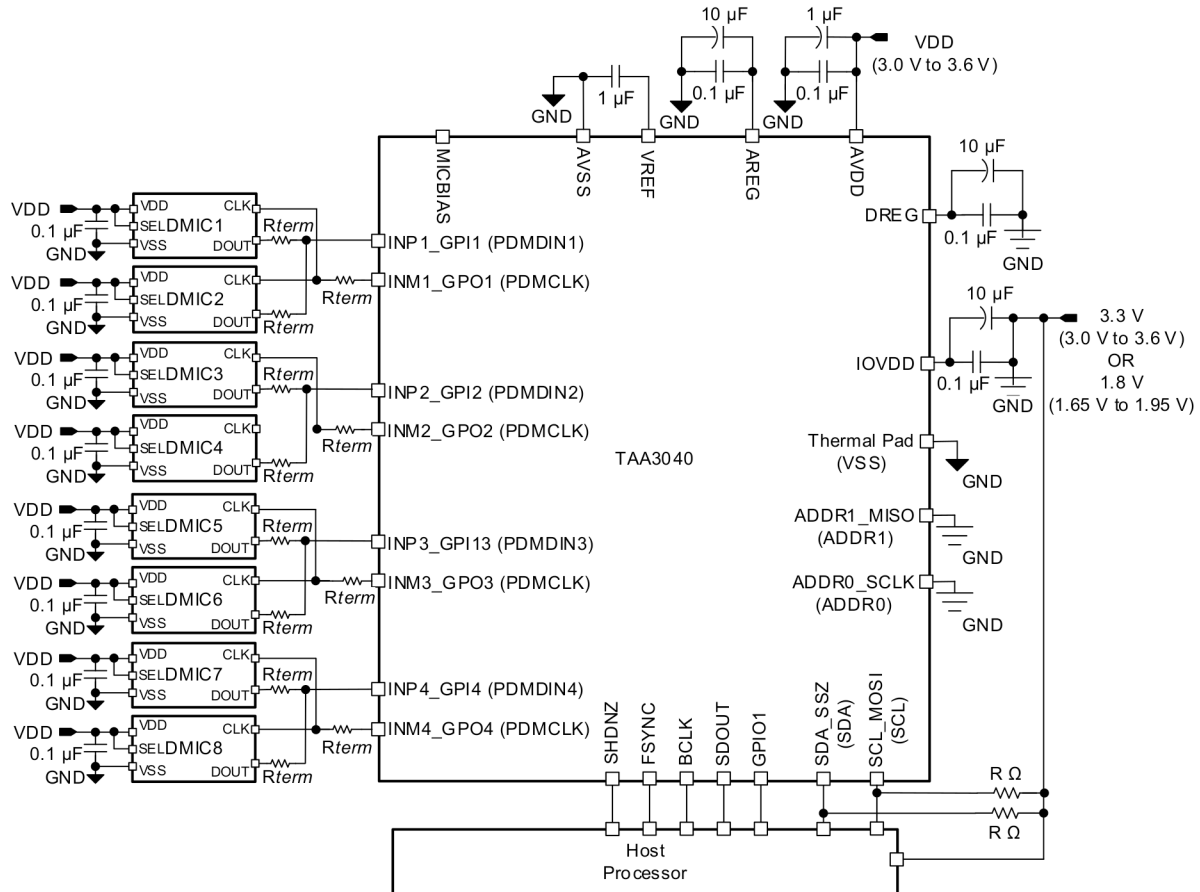
Figure 8-2. Eight-Channel Digital PDM Microphone Recording Diagram
