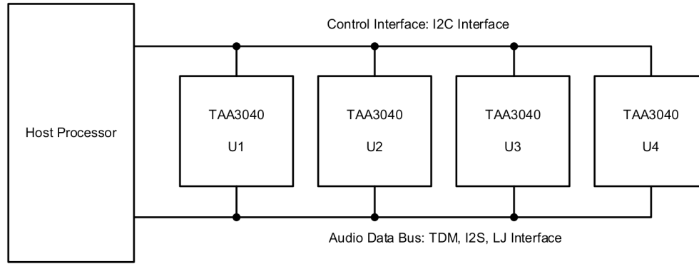
Figure 6-13. Multiple TAA3040 Devices With Shared Control and Audio Data Buses
