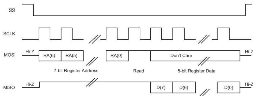
Figure 6-72. SPI Single-Byte Read Transfer
