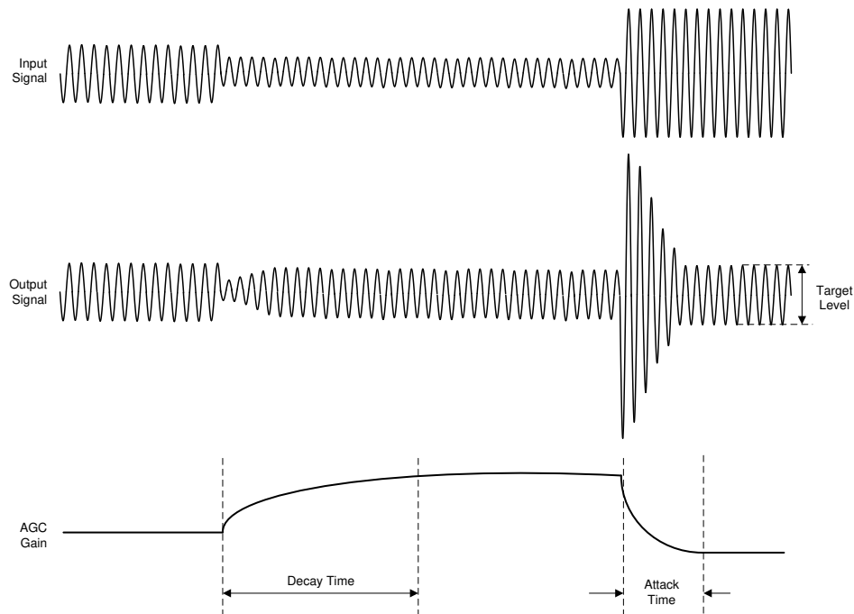
Figure 6-61. AGC Characteristics
