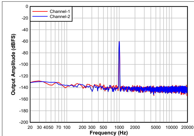
Figure 8-4. ADC FFT with -60dBFS Input
