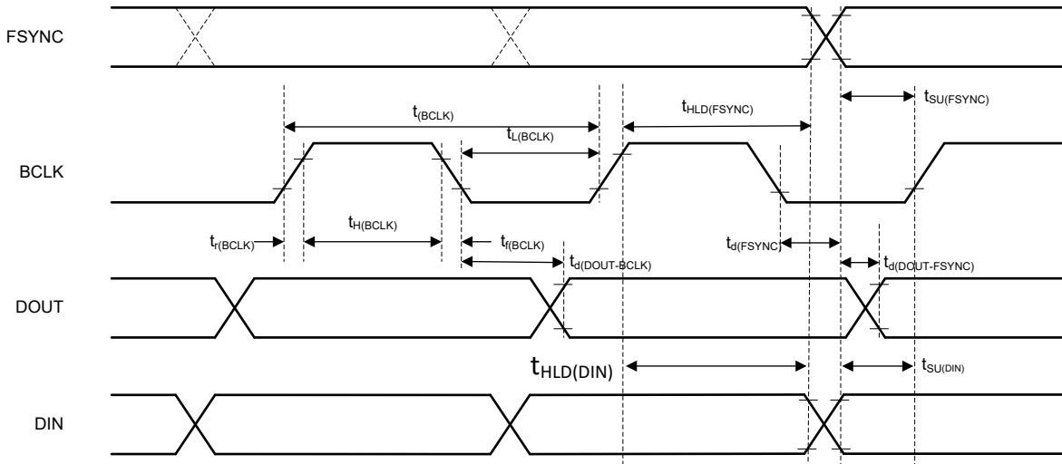
Figure 5-3. TDM, I 2 S, LJ Interface Timing Diagram
