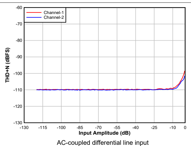
Figure 8-3. ADC THD+N Level vs Input
