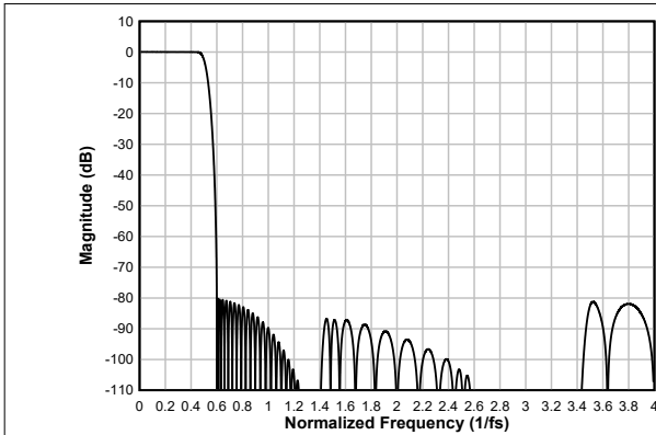
Figure 6-25. Linear-phase Decimation Filter Magnitude Response
