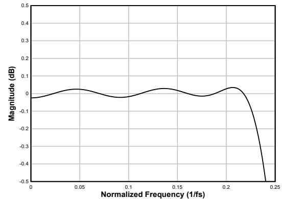
Figure 6-36. Linear-phase Decimation Filter Pass-Band Ripple
