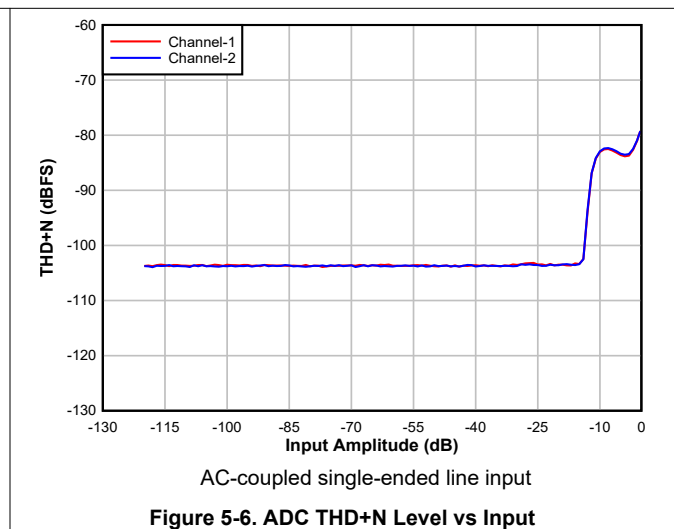
Figure 5-6. ADC THD+N Level vs Input
