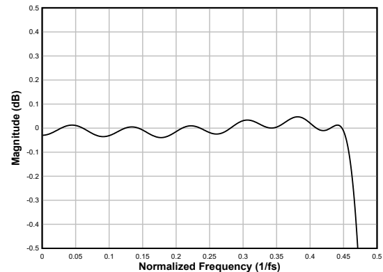
Figure 6-30. Linear-phase Decimation Filter Pass-Band Ripple
