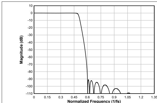
Figure 6-49. Low-latency Decimation Filter Magnitude Response
