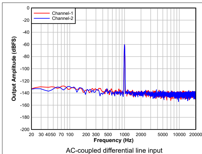
Figure 8-2. ADC FFT with -60dBFS Input
