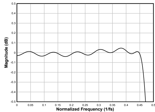
Figure 6-28. Linear-phase Decimation Filter Pass-Band Ripple
