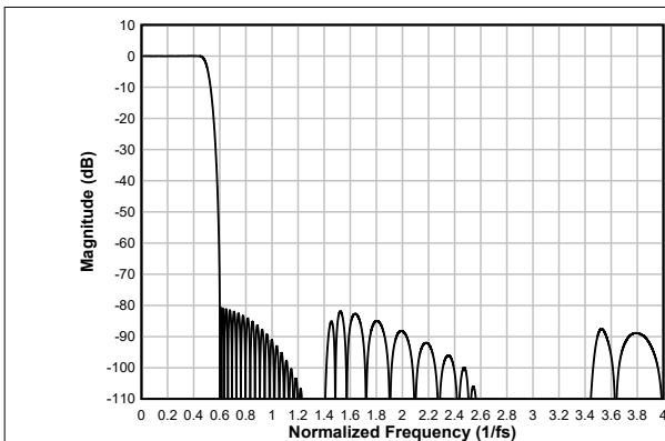
Figure 6-27. Linear-phase Decimation Filter Magnitude Response
