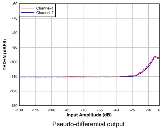
Figure 5-7. DAC THD+N Level vs Input
