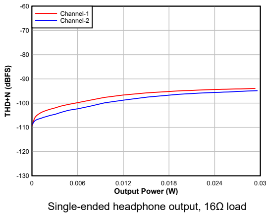
Figure 5-9. DAC THD+N Level vs output power
