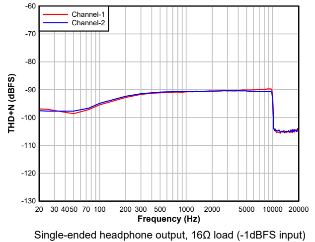
Figure 5-14. DAC THD+N Level vs Frequency
