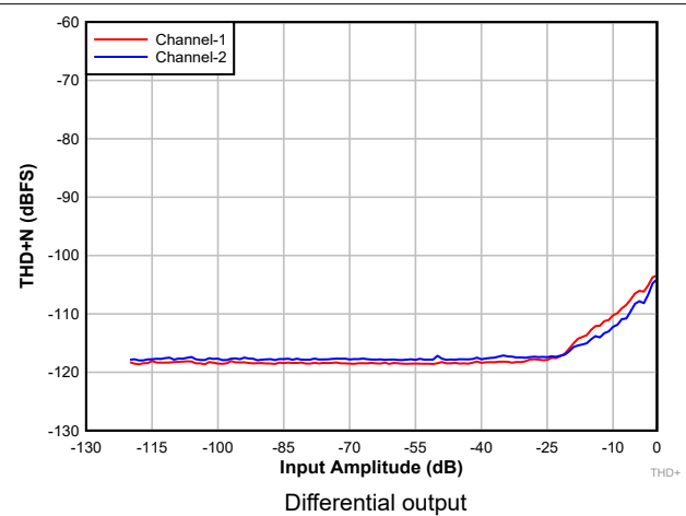
Figure 8-3. DAC THD+N Level vs Input
