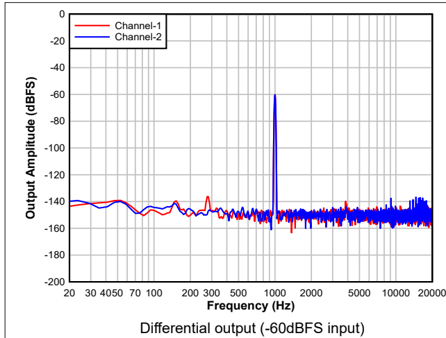
Figure 8-2. DAC FFT with -60dBFS Input
