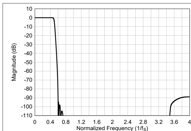
Figure 6-52. Ultra-Low-Latency interpolation Filter Magnitude Response
