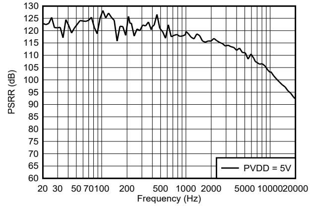
Figure 5-18. PVDD PSRR vs Frequency
