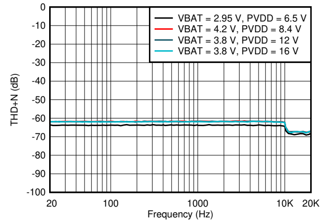
Figure 6-40. V Sense THDN vs Frequency
