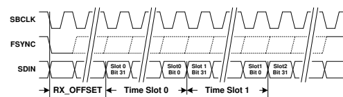
Figure 8-3. TDM RX Time Slots
