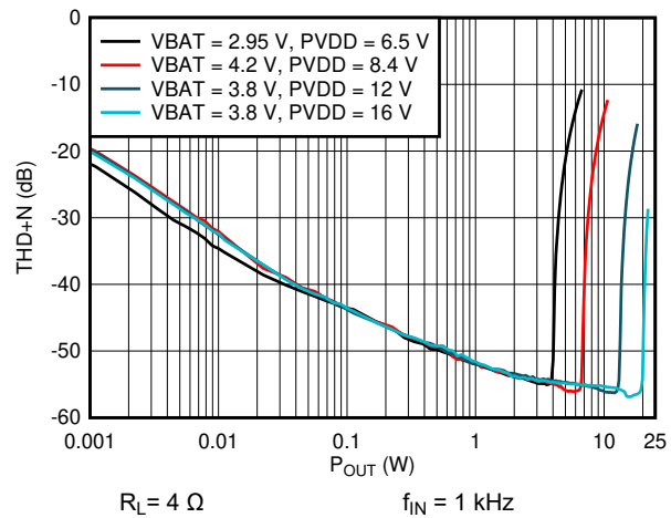
Figure 6-29. I Sense THDN vs Output Power
