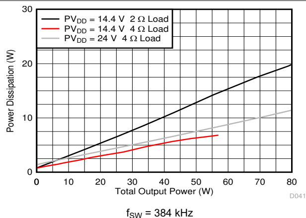
Figure 7-32. BTL Power Dissipation vs Total Output Power
