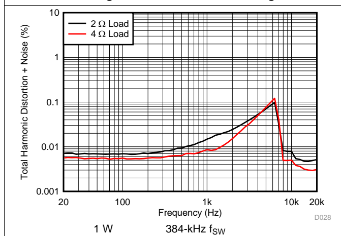
Figure 23. PBTL THD+N vs Frequency
