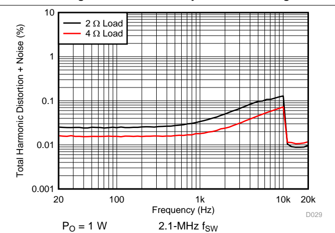
Figure 24. PBTL THD+N vs Frequency
