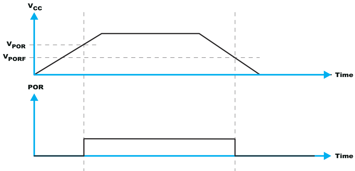
Figure 8-8. V_{POR}
