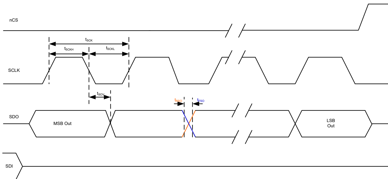
Figure 9-12. SPI AC Characteristic Read
