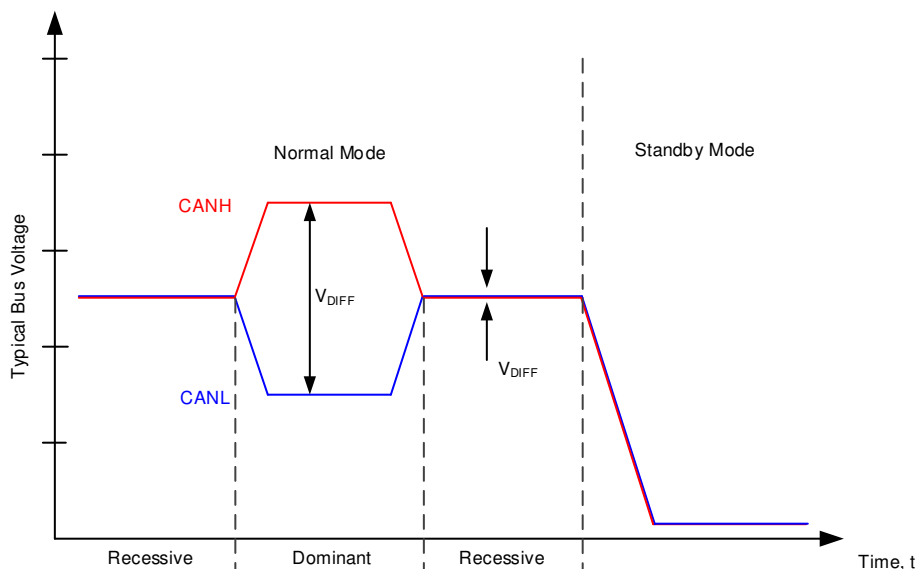
Figure 10-17. Bus States
