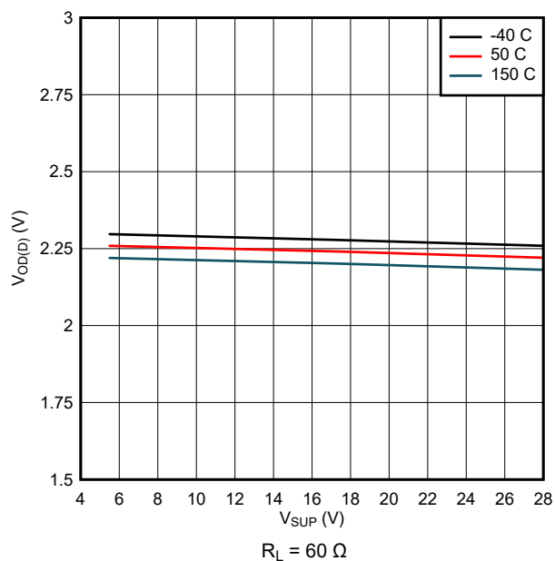
Figure 8-2. V_{OD(DOM)} over V_{SUP}
