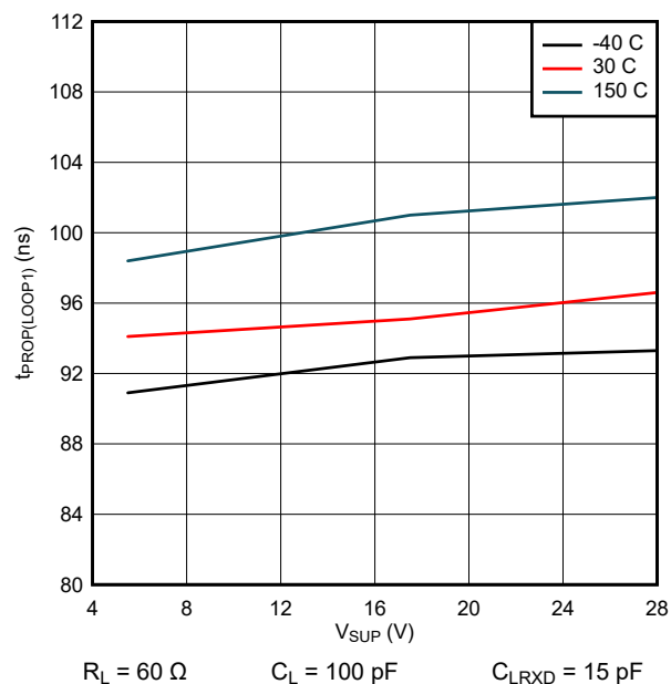
Figure 8-1. t_{pROP(LOOP1)} over V_{SUP}
