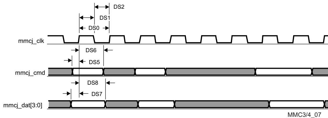
Figure 5-96. MMC/SD/SDIOj in - Default Speed - Receiver Mode
