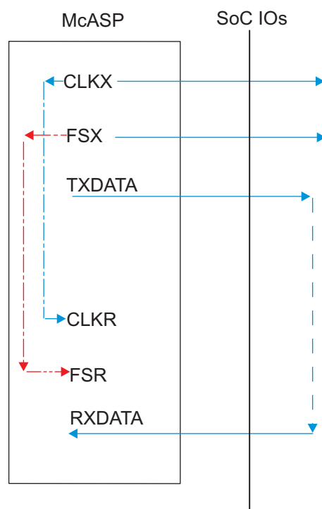
Figure 5-61. McASP1-8 CO-FO- – SYNC Mode
