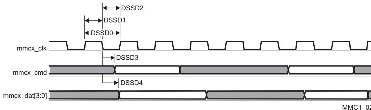
Figure 5-76. MMC/SD/SDIO in - Default Speed - Transmitter Mode
