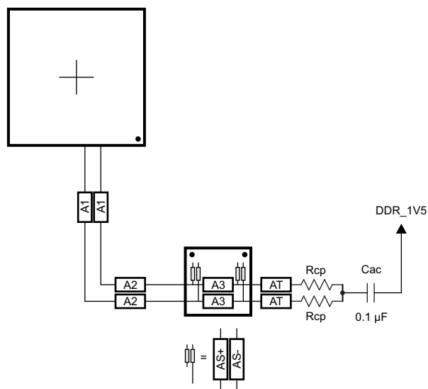
Figure 7-69. CK Routing for Two Mirrored DDR3 Devices
