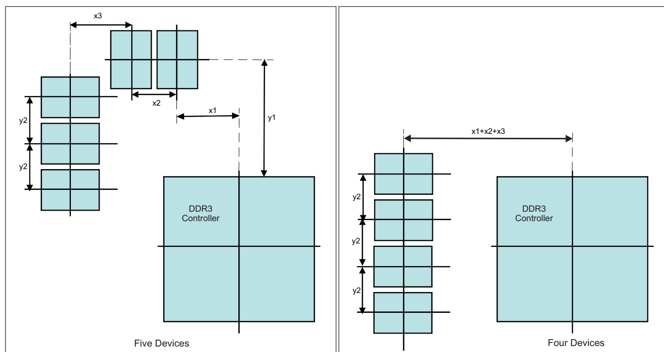
Figure 7-57. Placement Specifications
