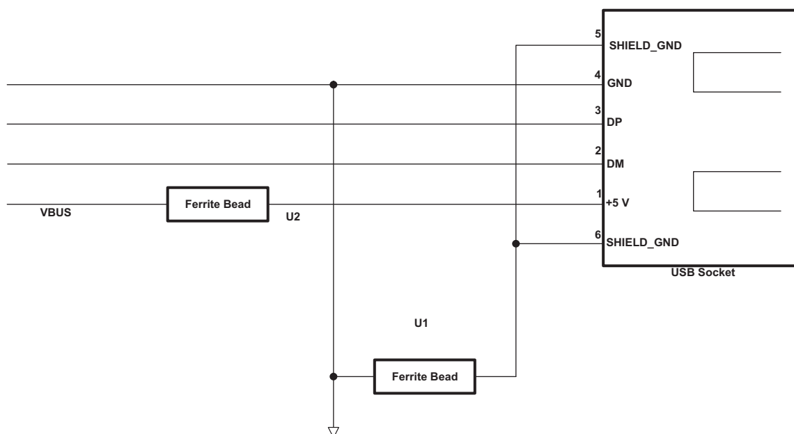
Figure 7-32. USB Connector
