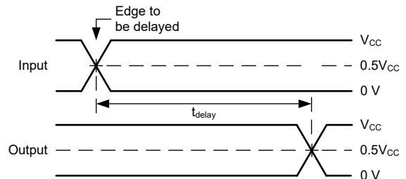
Figure 6-4. Voltage Waveforms, Edge Delay Time
