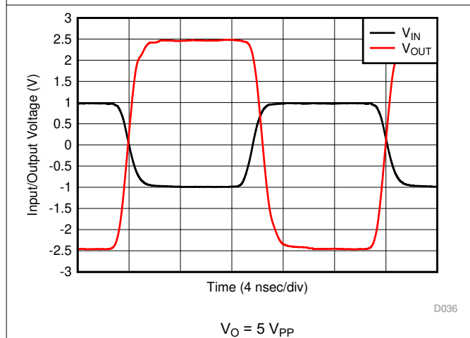
Figure 8-56. G = -5\text{ V/V} Pulse Response
