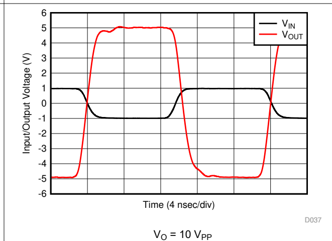
Figure 8-57. G = -5\text{ V/V} Pulse Response
