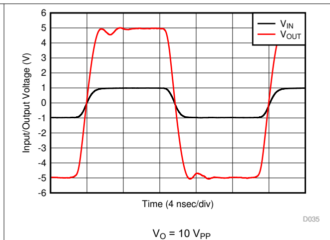
Figure 8-55. G = 5\text{ V/V} Pulse Response
