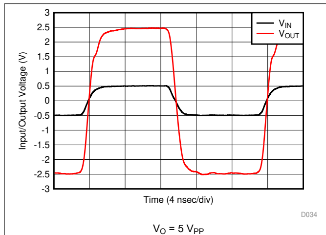
Figure 8-54. G = 5\text{ V/V} Pulse Response
