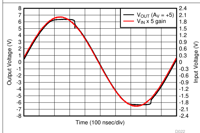
Figure 8-58. Overdrive Recovery Time
