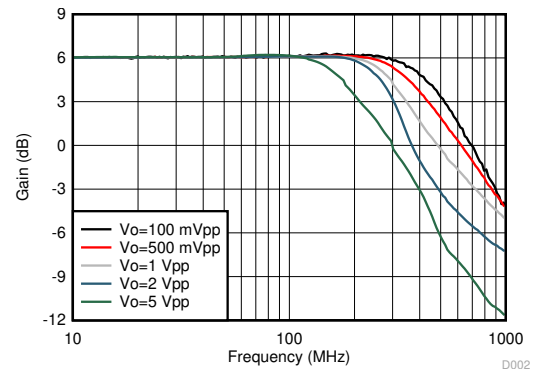
Figure 6-2. Frequency Response vs Vopp
