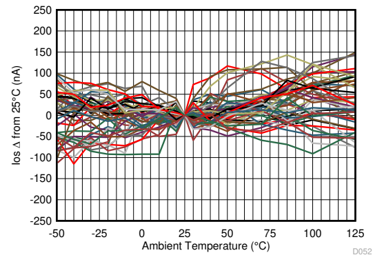
Figure 6-50. Input Offset Current
