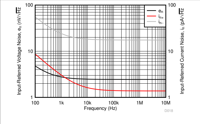
Figure 5-16. Input Voltage and Current Noise Density vs Frequency
