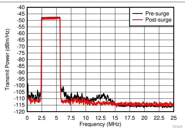
Figure 6-9. China SGCC HPLC Band1 Pre-Surge and Post-Surge
