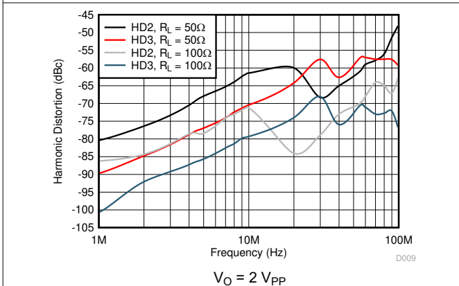
Figure 5-17. Harmonic Distortion vs Frequency
