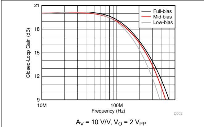
Figure 5-13. Small-Signal Frequency Response vs Bias Modes
