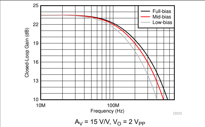
Figure 5-14. Small-Signal Frequency Response vs Bias Modes
