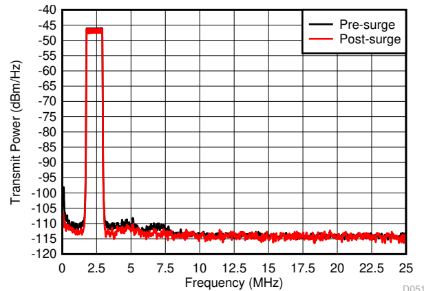
Figure 6-11. China SGCC HPLC Band3 Pre-Surge and Post-Surge
