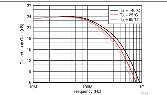
Figure 5-2. Large-Signal Frequency Response
