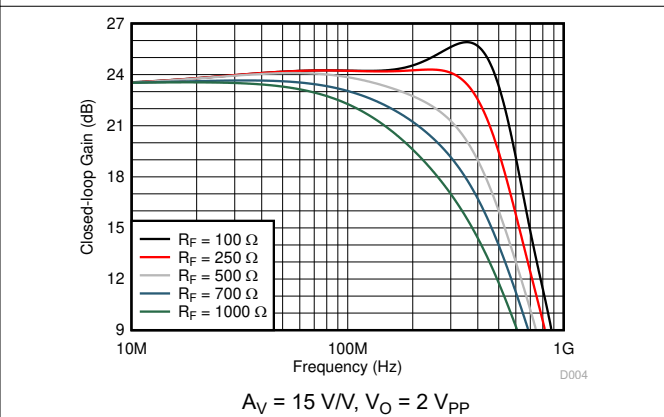
Figure 5-6. Small-Signal Frequency Response vs R_F
