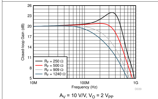
Figure 5-5. Small-Signal Frequency Response vs R_F
