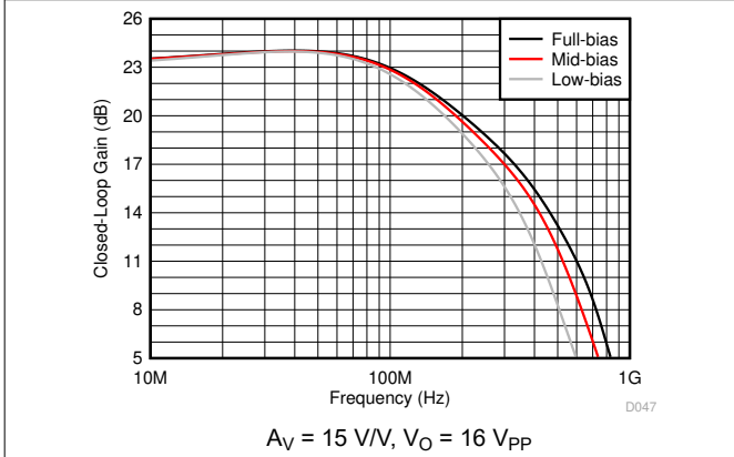
Figure 5-15. Large-Signal Frequency Response vs Bias Modes
