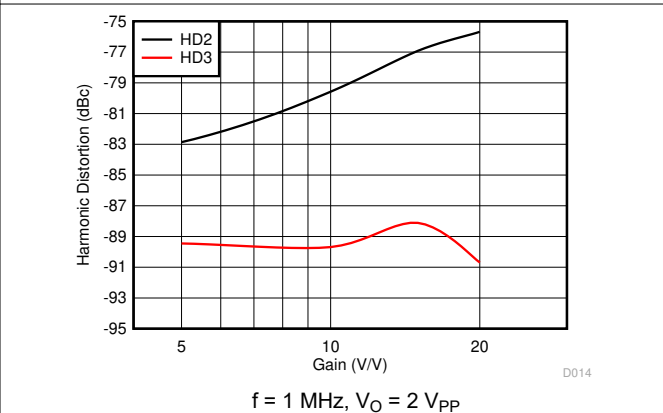
Figure 5-18. Harmonic Distortion vs Gain
