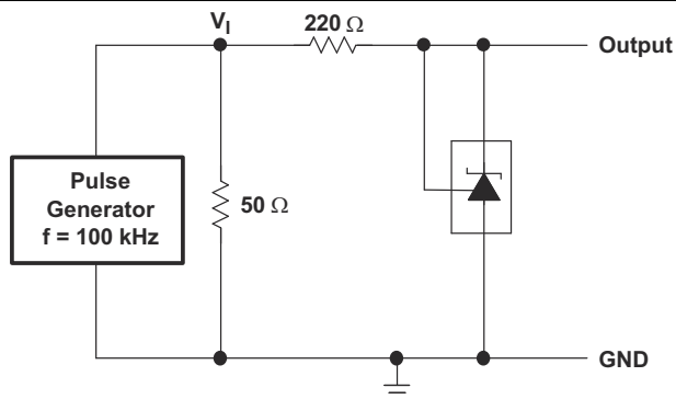
Figure 6-15. Test Circuit for Pulse Response
