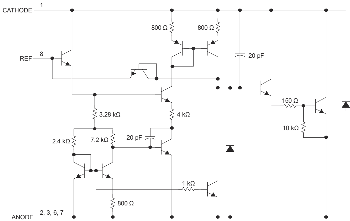
Figure 8-2. Equivalent Schematic
