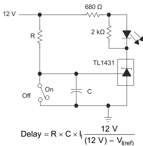
Figure 9-13. Delay Timer
