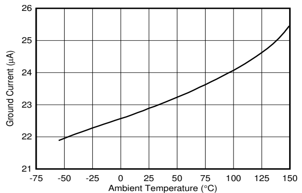
Figure 5-18. Ground Current at 500uA (New Chip)
