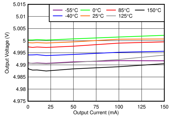
Figure 5-8. Load Regulation vs I_{OUT} (New Chip)
