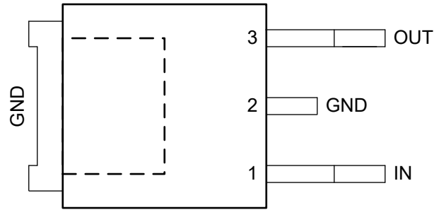
Figure 4-2. KVV Package, 3-Pin TO-252 (Top View)
