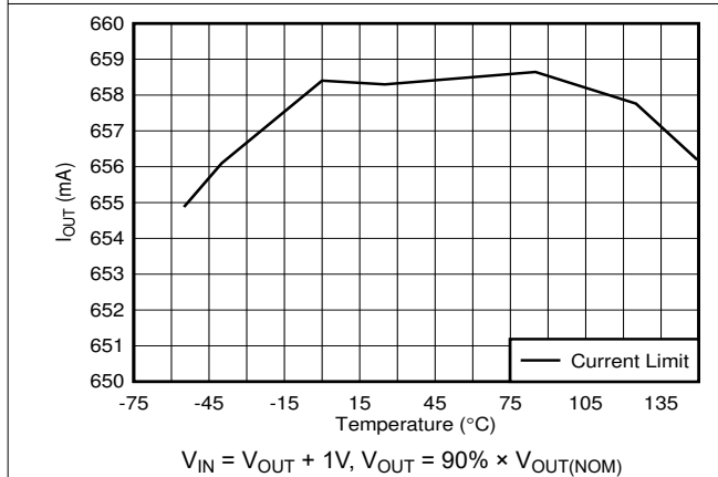
Figure 5-39. Output Current Limit vs Temperature (New Chip)
