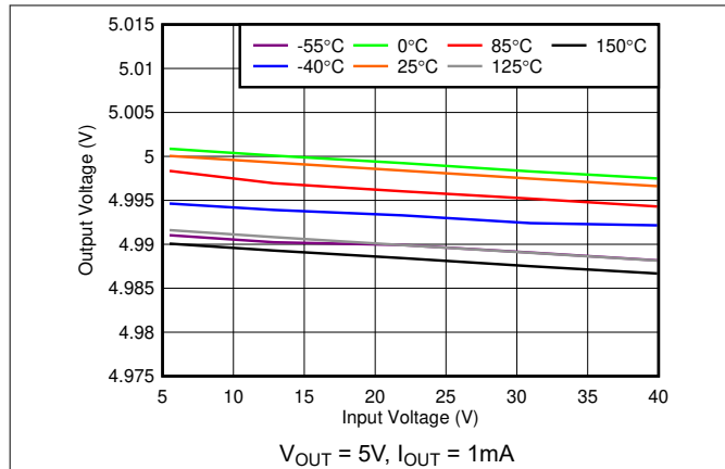
Figure 5-7. Line Regulation vs V_{IN} (New Chip)
