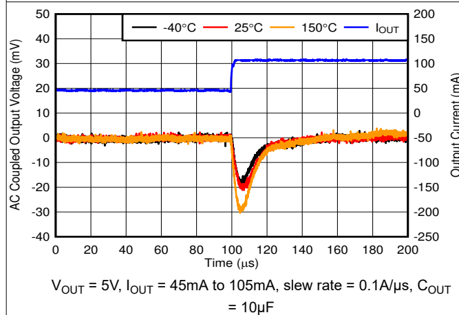
Figure 5-33. Load Transient, 45mA to 105mA Rising Edge (New Chip)
