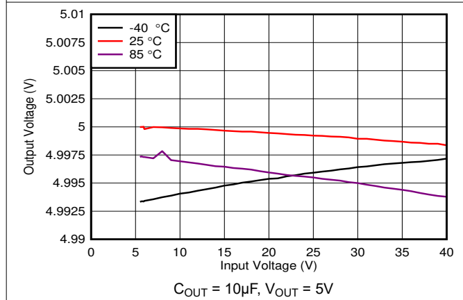
Figure 5-9. Line Regulation at 50mA (New Chip)
