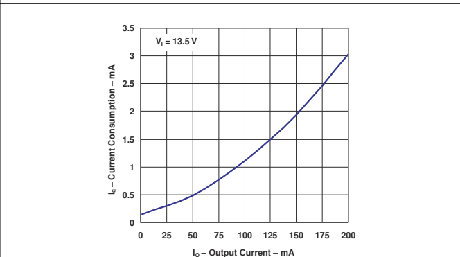
Figure 5-12. Current Consumption vs Output Current (Legacy Chip)
