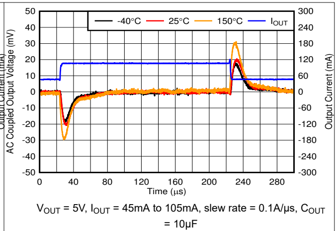
Figure 5-32. Load Transient, 45mA to 105mA (New Chip)
