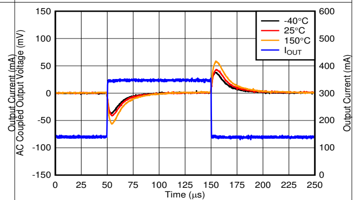
V_{OUT} = 5\text{V} , I_{OUT} = 150\text{mA} to 350\text{mA} , slew rate = 0.1\text{A}/\mu\text{s} , C_{OUT} = 10\mu\text{F}
