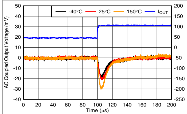
V_{OUT} = 5\text{V} , I_{OUT} = 45\text{mA} to 105\text{mA} , slew rate = 0.1\text{A}/\mu\text{s} , C_{OUT} = 10\mu\text{F}
