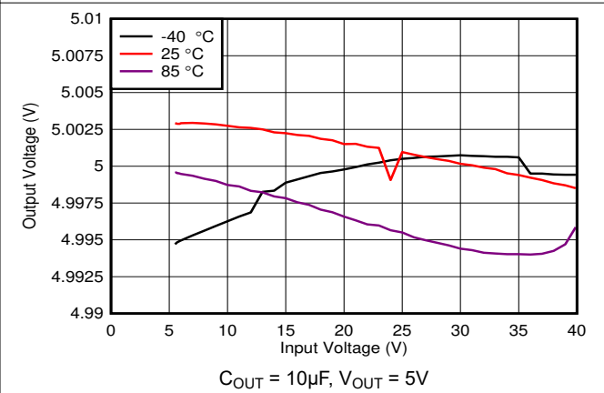
Figure 5-10. Line Regulation at 100mA (New Chip)
