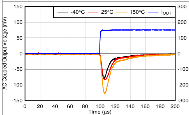
V_{OUT} = 5\text{V} , I_{OUT} = 0\text{mA} to 150\text{mA} , slew rate = 1\text{A}/\mu\text{s} , C_{OUT} = 10\mu\text{F}
