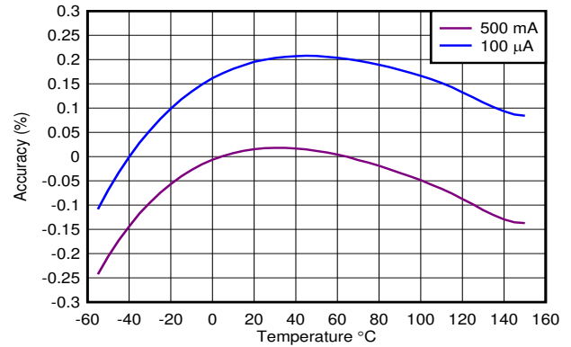
Figure 5-4. Output Accuracy vs Temperature (New Chip)
