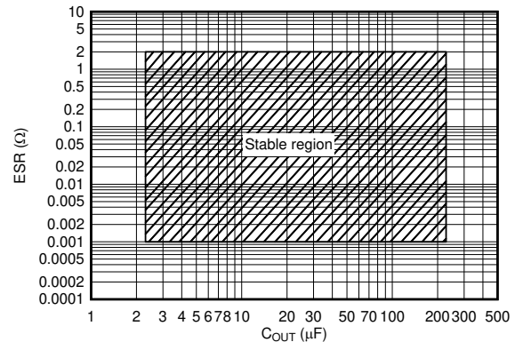
Figure 5-46. Stability, ESR vs C_{OUT} (New Chip)
