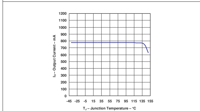
Figure 5-11. Output Current vs Junction Temperature (Legacy Chip)
