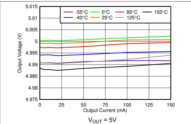
Figure 5-8. Load Regulation vs I_{OUT} (New Chip)
