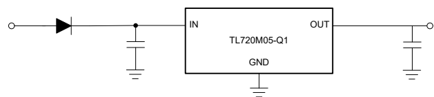
Typical Application Schematic (New Chip)
