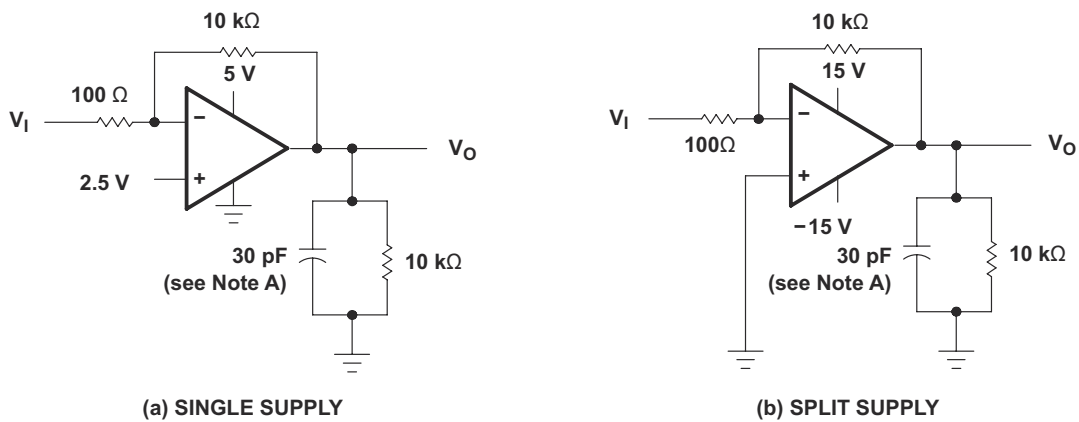
Figure 6-2. Noise-Voltage Test Circuit
