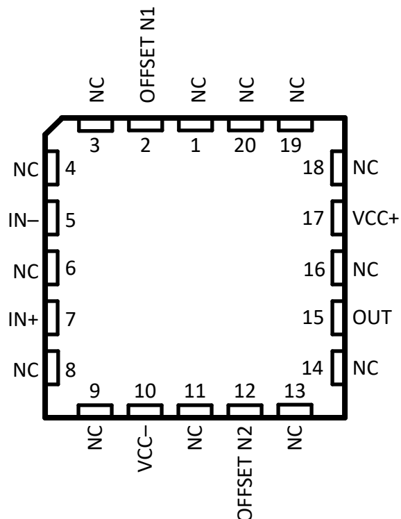
Figure 5-6. TLE2071M and TLE2071AM FK PACKAGE (Top View)
