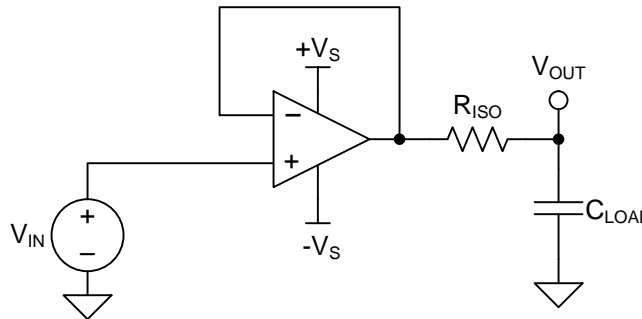
Figure 35. Unity-Gain Buffer With R_{\text{ISO}} Stability Compensation
