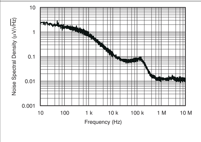
Figure 6-12. Spectral Noise Density vs Frequency
