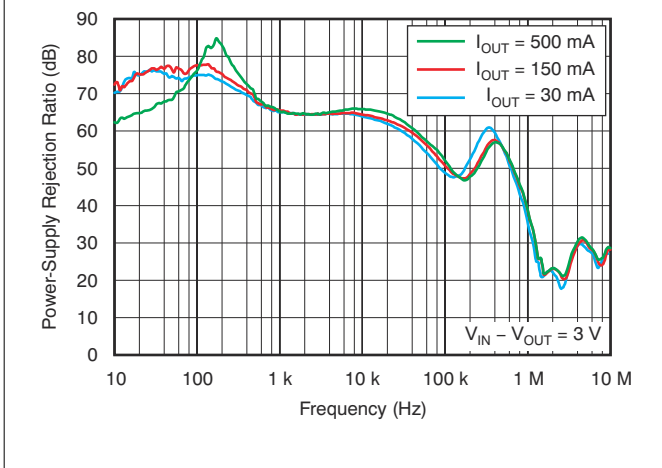
Figure 6-9. Power-Supply Rejection Ratio vs Frequency
