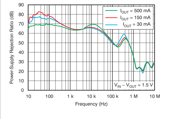
Figure 6-10. Power-Supply Rejection Ratio vs Frequency
