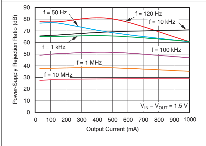
Figure 6-11. Power-Supply Rejection Ratio vs Output Current
