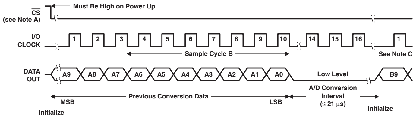
Figure 9. Timing for 16-Clock Transfer Not Using \overline{\text{CS}} (Serial Transfer Completed Within 21 μs)
