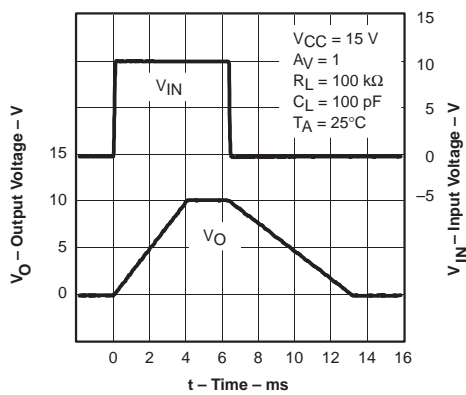
LARGE SIGNAL FOLLOWER PULSE RESPONSE
