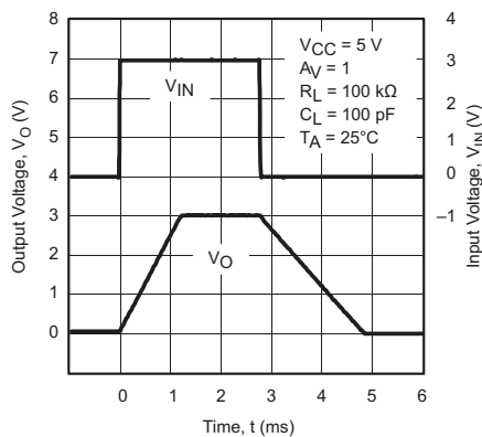
Figure 29. Large Signal Follower Pulse Response
