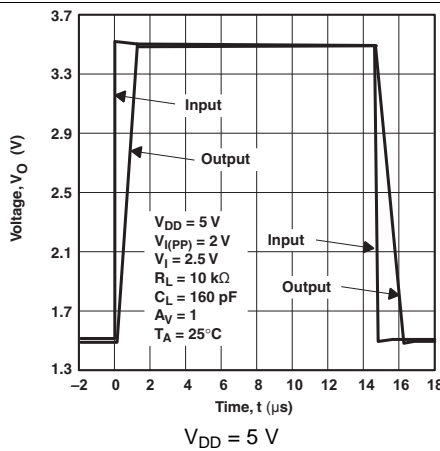
Figure 41. Large Signal Follower
