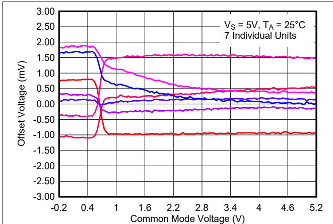
Figure 6-48. Offset Voltage vs. Common Mode Voltage, 5 V
