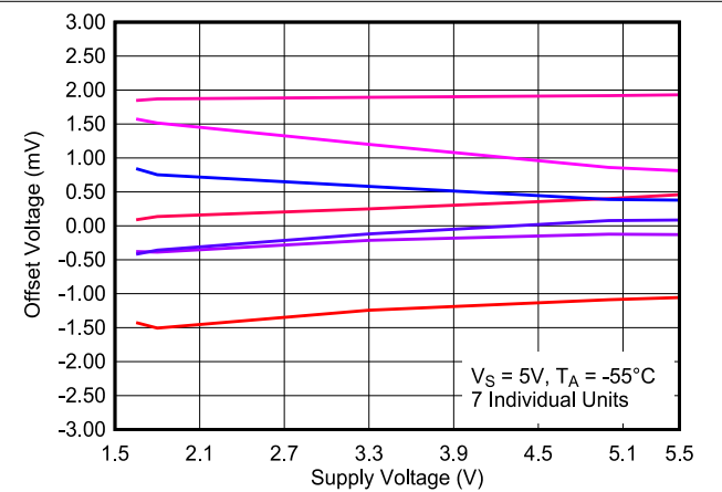
Figure 6-51. Offset Voltage vs. Supply Voltage, -55°C
