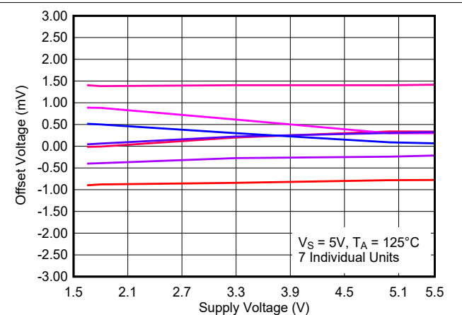
Figure 6-49. Offset Voltage vs. Supply Voltage, 125°C
