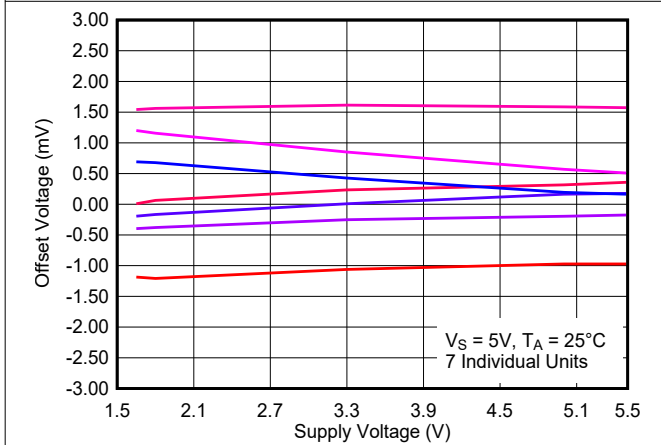
Figure 6-50. Offset Voltage vs. Supply Voltage, 25°C
