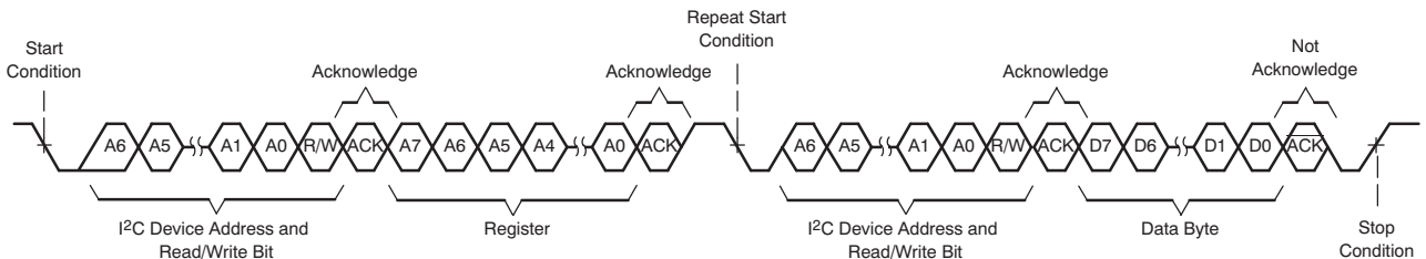
Figure 91. I 2 C Single-Byte Read Transfer
