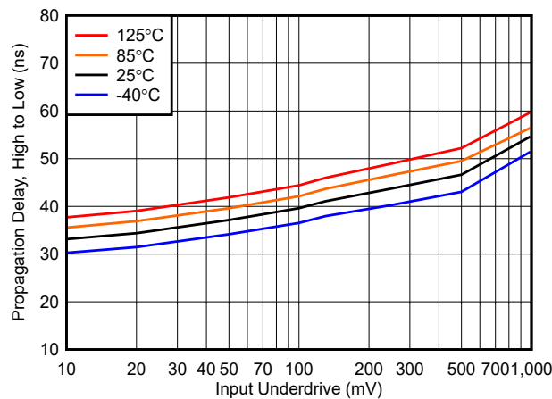
Figure 5-35. Propagation Delay, High to Low vs. Underdrive at 5V
