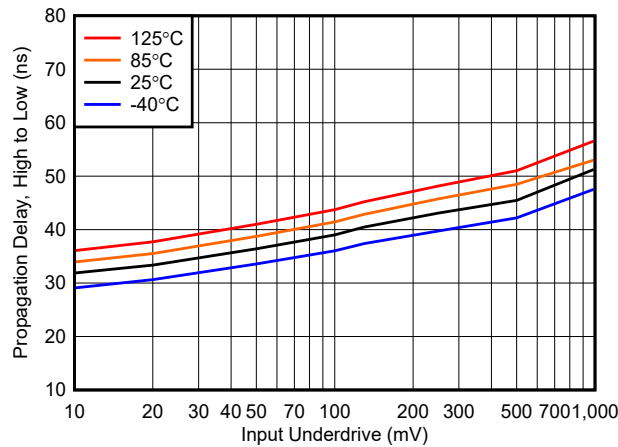
Figure 5-33. Propagation Delay, High to Low vs. Underdrive at 3.3V
