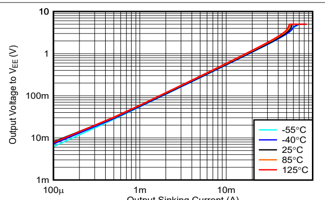
Figure 5-22. Output Voltage vs. Output Sinking Current, 5V
