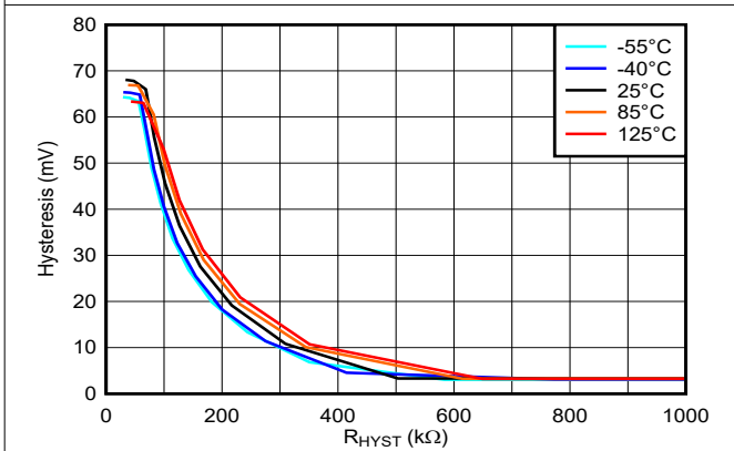
Figure 5-11. Hysteresis vs. Resistance, 2.5V
