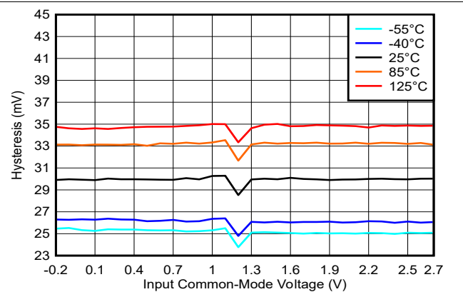
Figure 5-6. Hysteresis vs. Common-Mode, 2.5V
