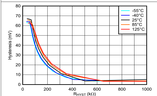
Figure 5-13. Hysteresis vs. Resistance, 5V
