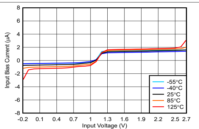
Figure 5-14. Bias Current vs. Input Voltage, 2.5V
