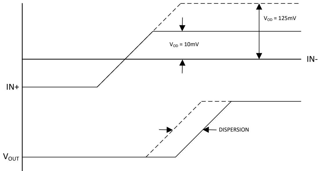
Figure 5-2. Overdrive Dispersion
