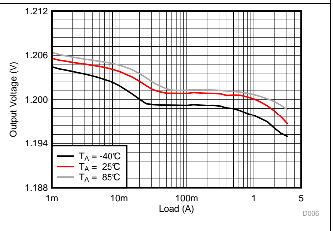
Figure 10. Load Regulation
