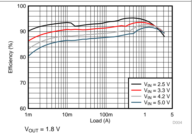
Figure 8. Efficiency
