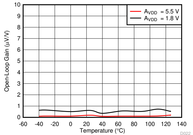
Figure 7-22. Open-Loop Gain vs Temperature
