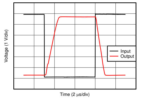
Figure 7-30. Overload Recovery
