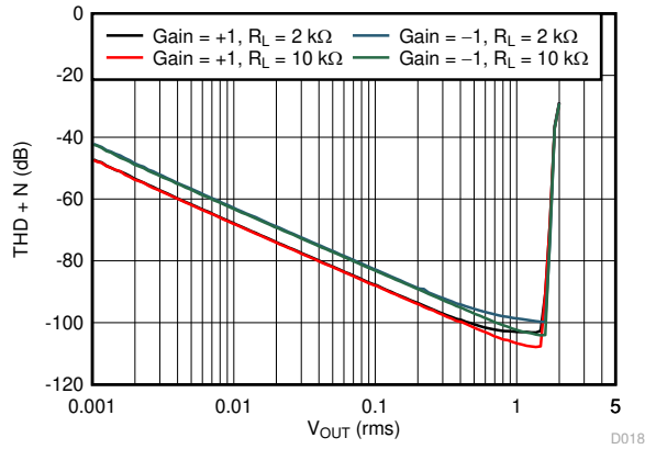
Figure 7-19. THD + N vs Amplitude
