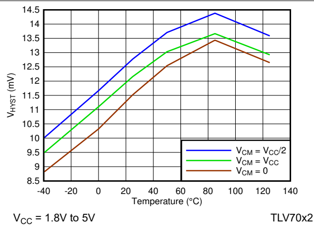
Figure 5-13. Hysteresis vs Temperature
