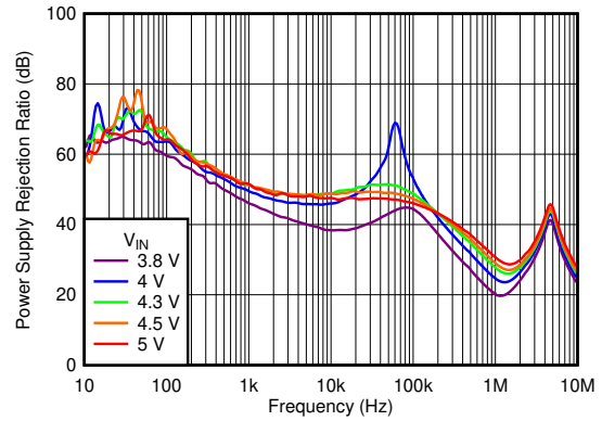
Figure 5-2. PSRR vs Frequency and V_{IN} V_{OUT} = 3.3\text{V} , C_{OUT} = 1\mu\text{F} , I_{OUT} = 500\text{mA}
