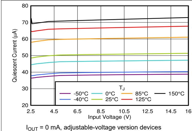
Figure 7-5. I_Q vs V_{IN}
