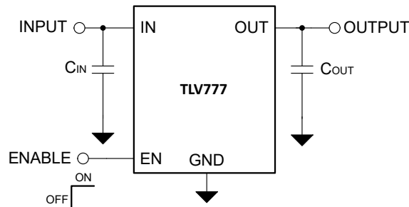
Figure 7-1. TLV777 Typical Application
