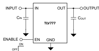
Typical Application Circuit
