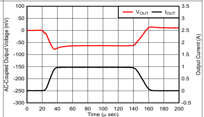
Figure 5-10. Current Limit
