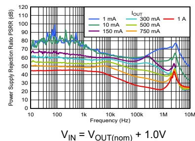
Figure 3-1. PSRR vs Frequency
