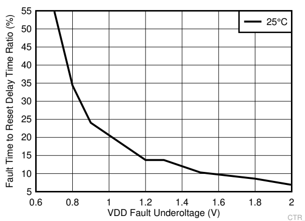
Figure 8-3. C_{CT} Discharge Time During Fault Condition ( V_{IT-} = 2.1\text{ V} , C_{CT} = 1\text{ }\mu\text{F} )
