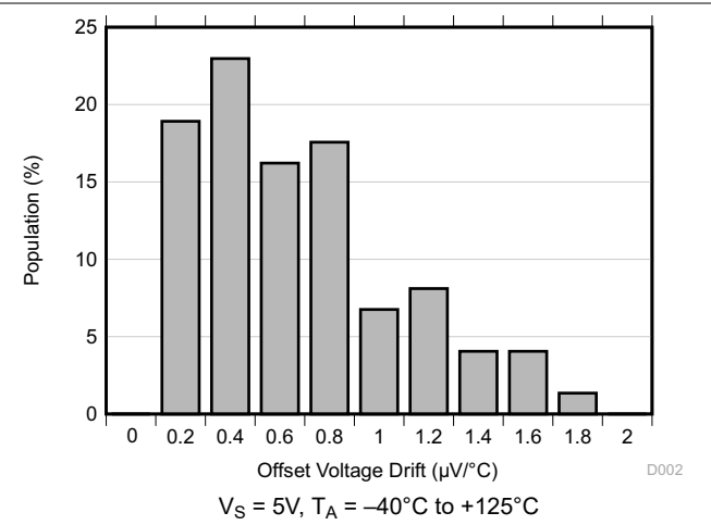
Figure 6-2. Offset Voltage Drift Distribution Histogram
