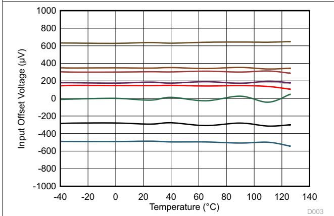
Figure 6-3. Input Offset Voltage vs Temperature
