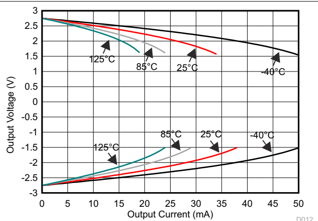
Figure 6-12. Output Voltage vs Output Current (Claw)
