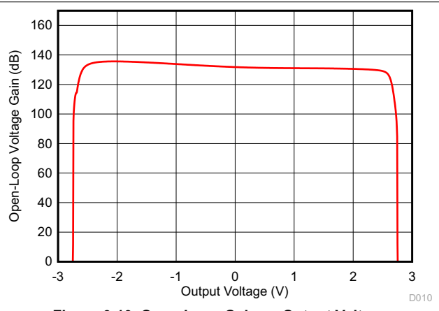
Figure 6-10. Open-Loop Gain vs Output Voltage
