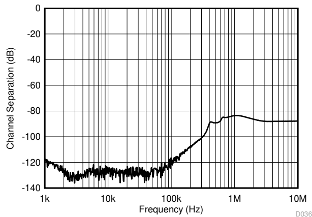
D036 Figure 6-36. Channel Separation
