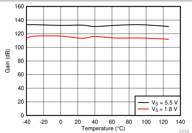
Figure 6-8. Open-Loop Gain vs Temperature
