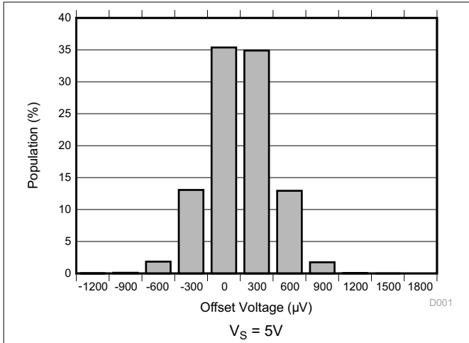
Figure 6-1. Offset Voltage Distribution Histogram
