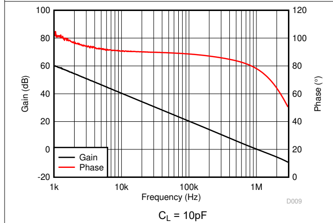
Figure 6-9. Open-Loop Gain and Phase vs Frequency
