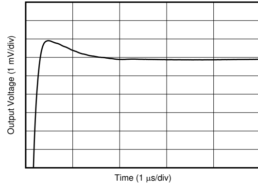
D032 G = 1 C_L = 100\text{pF} 2\text{V step}
