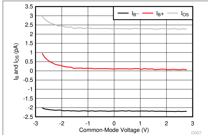
Figure 6-7. I_B and I_{OS} vs Common-Mode Voltage
