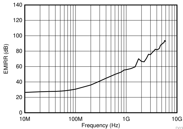
D035 Figure 6-35. Electromagnetic Interference Rejection Ratio Referred to Noninverting Input (EMIRR+) vs Frequency
