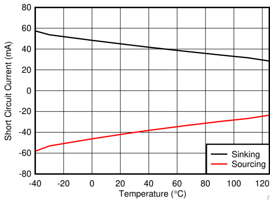
D033 Figure 6-33. Short-Circuit Current vs Temperature
