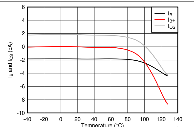
Figure 6-6. I_B and I_{OS} vs Temperature
