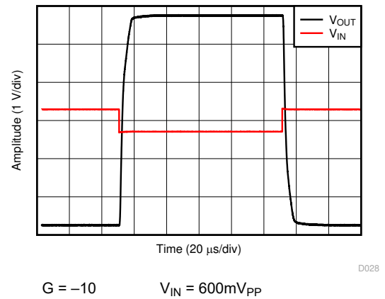
Figure 6-28. Overload Recovery
