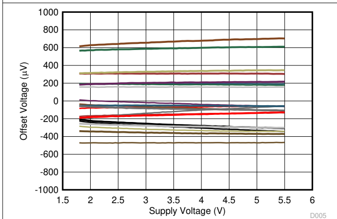
Figure 6-5. Offset Voltage vs Supply Voltage
