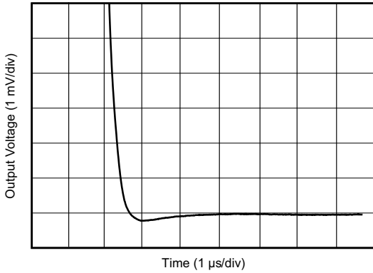
D031 G = 1 C_L = 100\text{pF} 2\text{V step}
