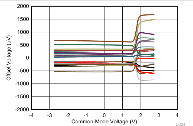
Figure 6-4. Offset Voltage vs Common-Mode
