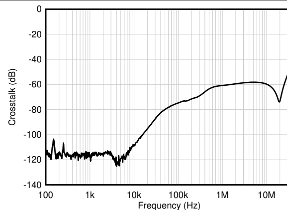
Figure 7-46. Channel Separation
