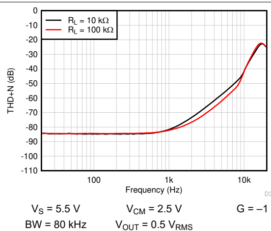
Figure 7-24. THD + N vs Frequency
