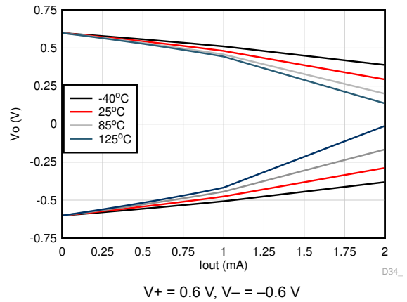
Figure 7-16. Output Voltage vs Output Current (Claw)
