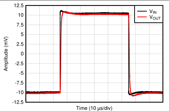
Figure 7-32. No Phase Reversal
