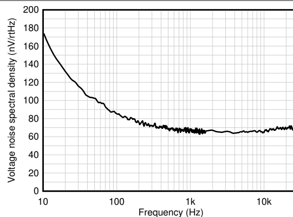
Figure 7-22. Input Voltage Noise Spectral Density
