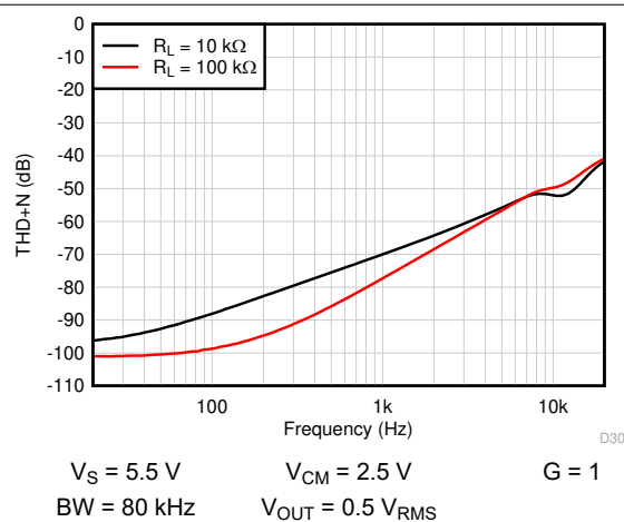
Figure 7-23. THD + N vs Frequency
