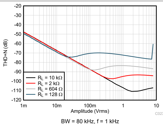
Figure 6-22. THD+N vs Output Amplitude
