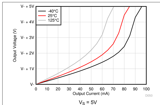
Figure 5-19. Output Voltage Swing vs Output Current (Sinking)
