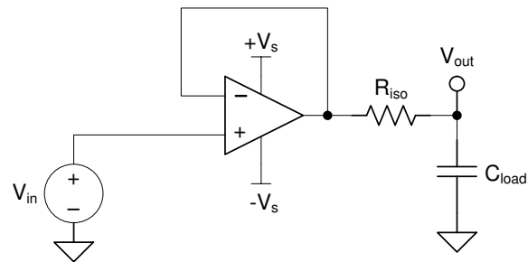
Figure 6-7. Extending Capacitive Load Drive With the TLV9161-Q1
