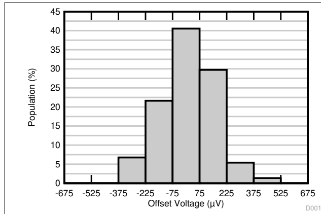
Distribution from 74 amplifiers, T_A = 25^\circ\text{C}
