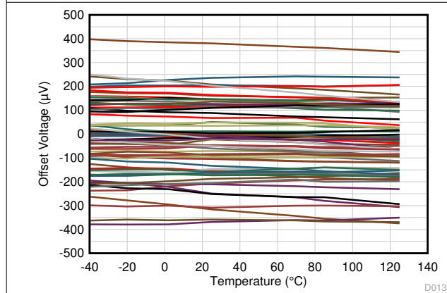
V_{CM} = V_- Data from 74 amplifiers
