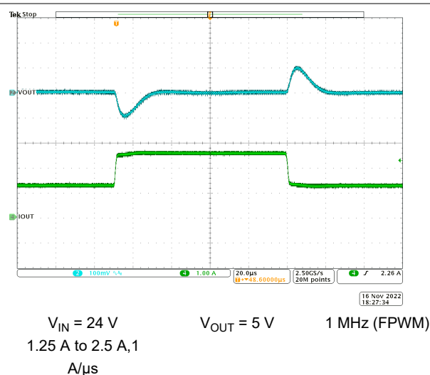
Figure 8-13. Load Transient
