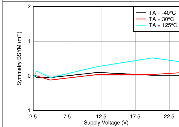
Figure 6-21. B_{SYM(X)} vs V_{CC}
