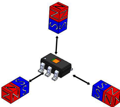
Figure 7-4. Axis Polarities
