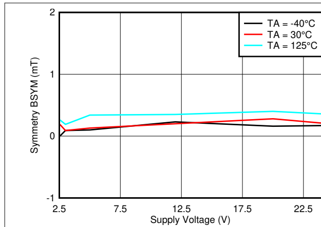
Figure 6-19. B_{SYM(Z)} vs V_{CC}
