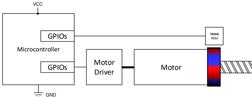
Figure 8-1. Incremental Encoding
