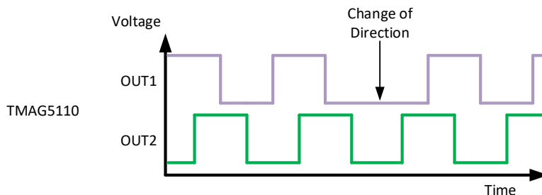
Figure 8-2. TMAG5110-Q1 Output Response
