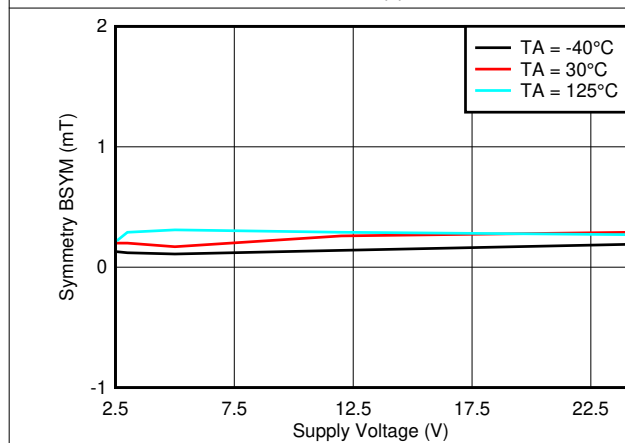
Figure 6-23. B_{SYM(Y)} vs V_{CC}
