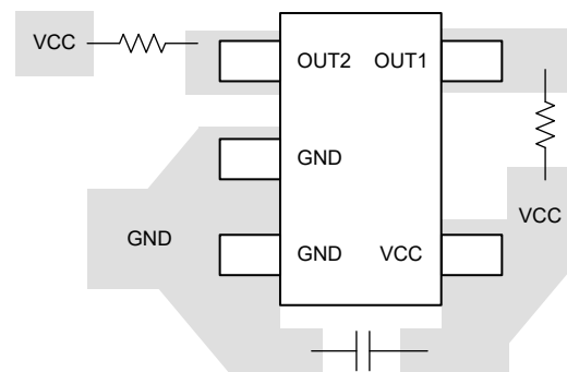
Figure 8-5. Layout Example (Pinout Version: R)
